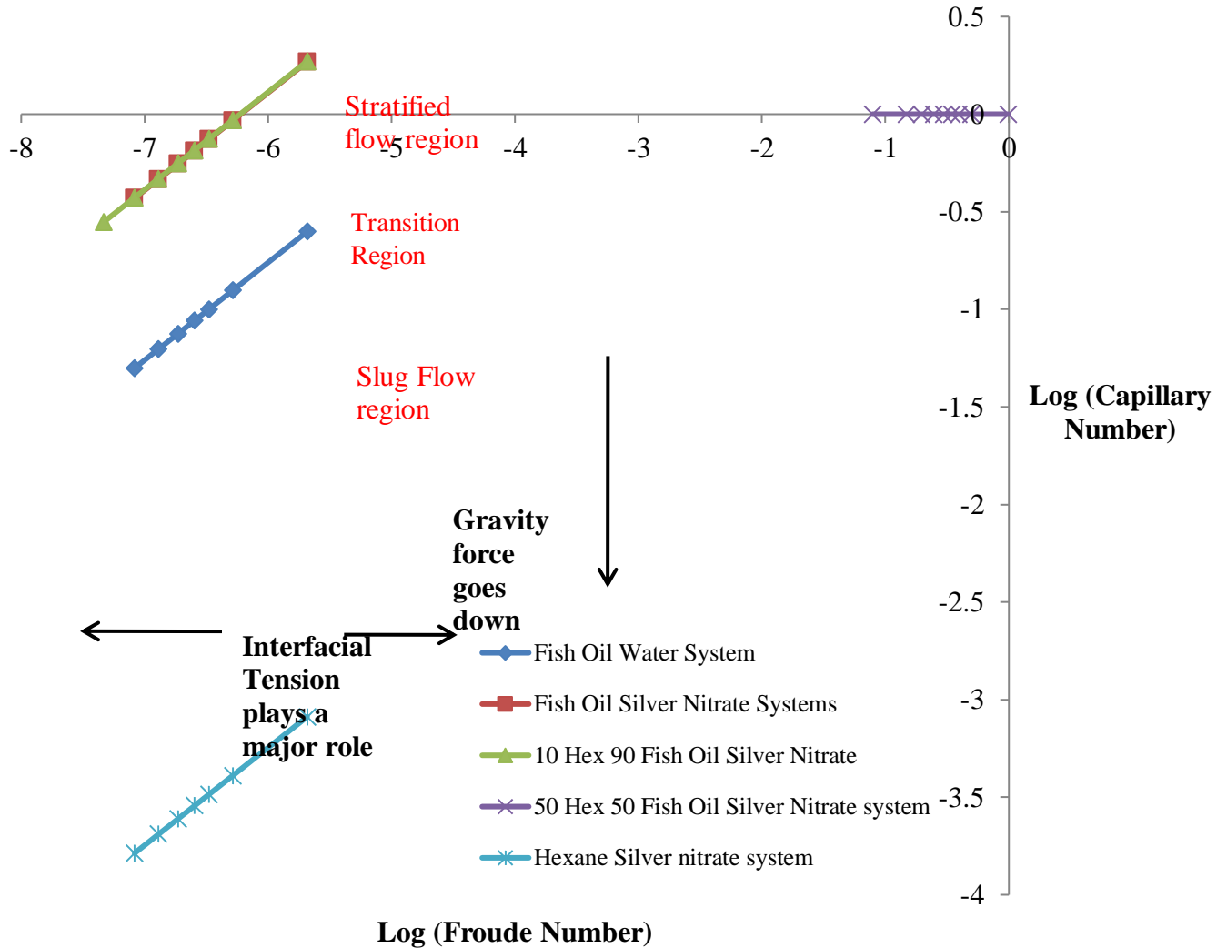
Fig. 5. The plot between Log (Ca) vs. Log (Fr) for fish oil water system, fish oil AgNO 3 system, 10 Hex 90 Fish Oil AgNO 3 systems, 50% Hex 50 % Fish Oil AgNO 3 system, and Hexane AgNO 3 system flow in 1/16th inch ID of PFA mini-channel is shown below.
