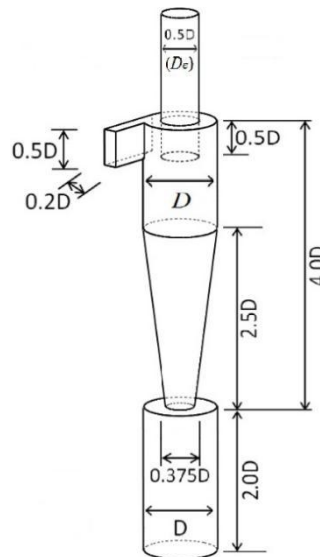
Fig. 1 Geometric details of cyclone model ( D = 0.205 m)
