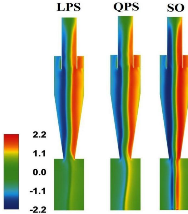
Fig. 5 Contour plots on Y/D=0 plane at U_{in} = 16.1 m/s. of mean tangential velocity.
