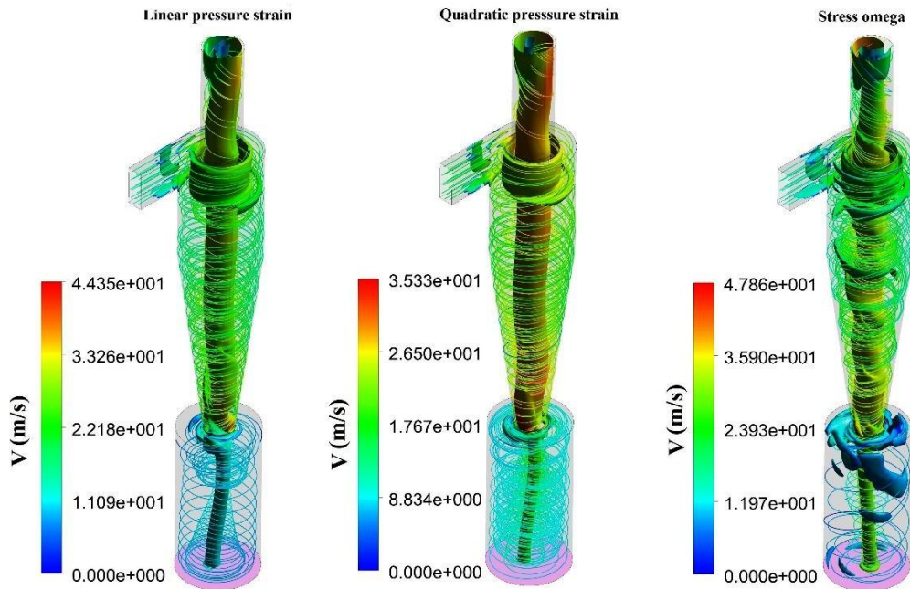
Fig. 11 Vortex core and streamlines representation for all the sub- models at inlet velocities, U_{in} = 16.1 m/s.
