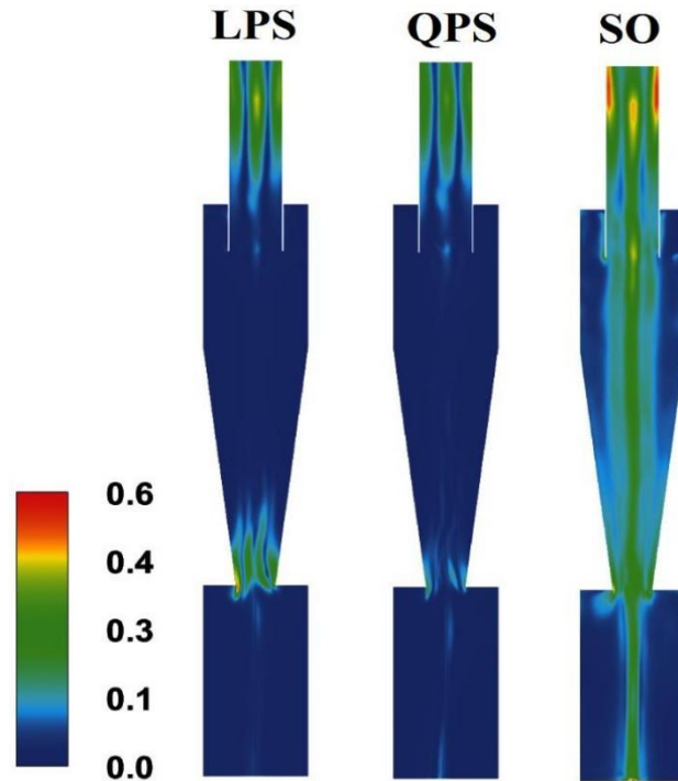
Fig. 7 Contour plots on Y/D=0 plane at U_{in} = 16.1 m/s. of rms tangential velocity.
