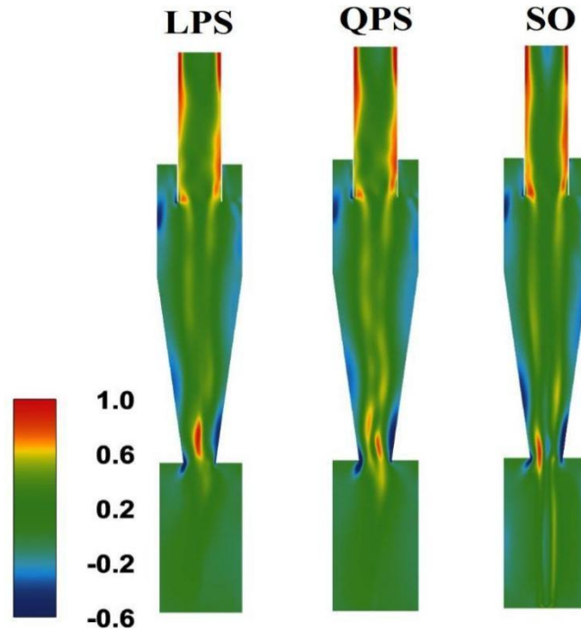
Fig. 3 Contour plots on Y/D=0 plane at U_{in} = 16.1 m/s. of mean axial velocity.
