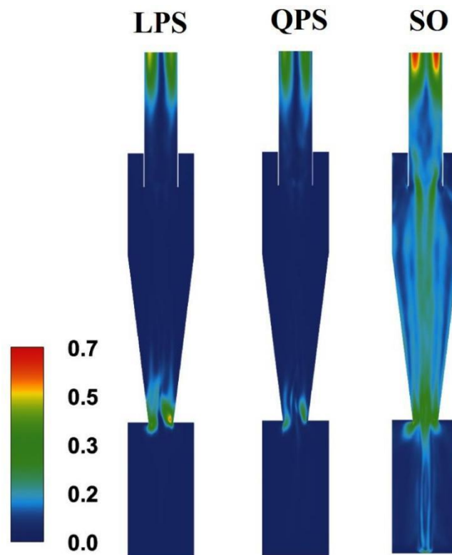
Fig. 9 Contour plots on Y/D=0 plane at U_{in} = 16.1 m/s. of rsm axial velocity.
