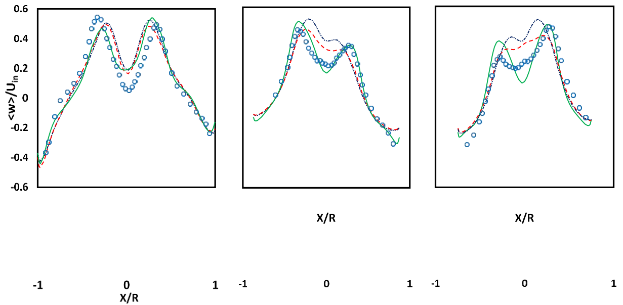
Fig. 4 From left to right: the radial profiles at z/D=0.75, 2.0, and 2.5 of mean axial velocity.
