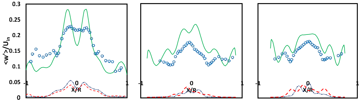
Fig. 10 From left to right: the radial profiles at z/D=0.75, 2.0, and 2.5 of rms axial velocity.
