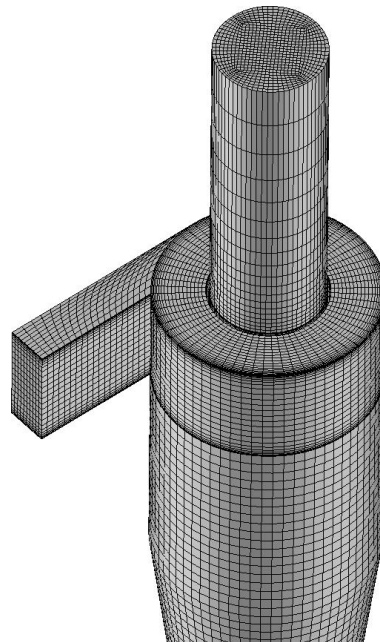
Fig. 2 Details of the mesh containing nearly 385K hexahedra of Stairmand high efficiency cyclone model
