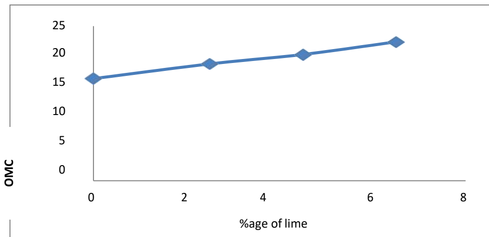
Figure 7.Variation of OMC of soil samples having different percentages of lime
