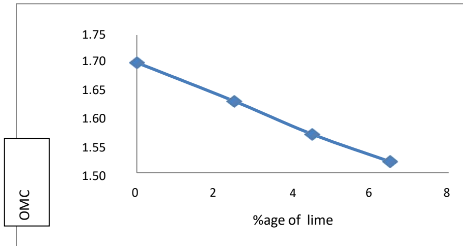
Figure6. Variation of OMC of soil samples having different percentages of lime
