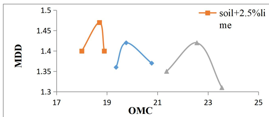
Figure 5. Variation of Maximum dry density of soil having different Percentages of calcium hydroxide with various percentages of sodium silicate as 1.5%, 2.5% and 3.5% respectively
